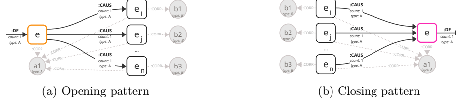
Fig. 3: Causal Event Relationships
